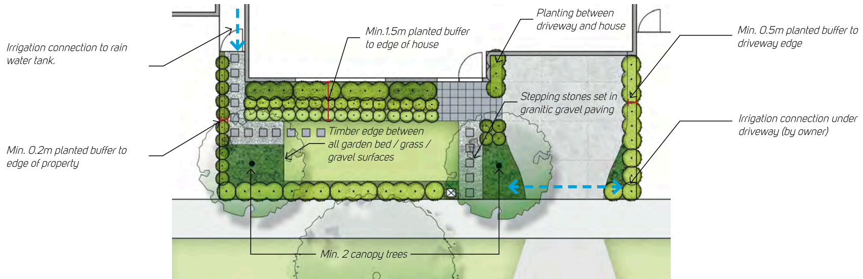
Standard Lot - typical minimum requirements (layout will vary depending on chosen design)
