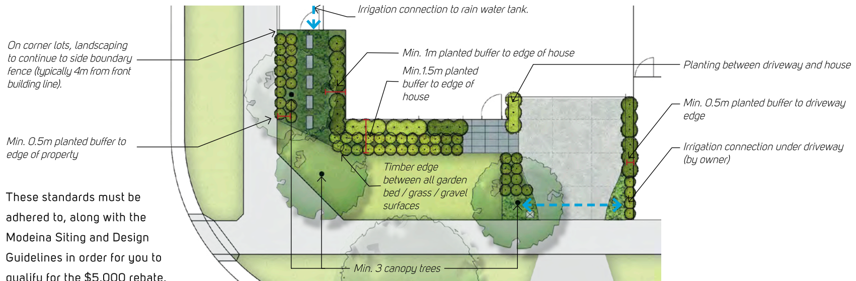
Corner Lot - typical minimum requirements (layout will vary depending on chosen design)
